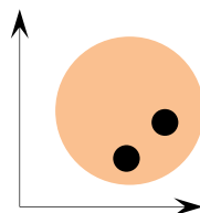
One molecule
