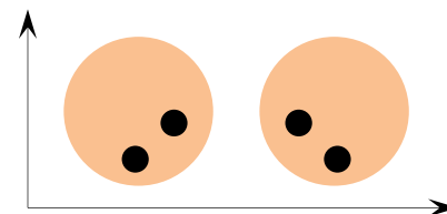
Two molecules
